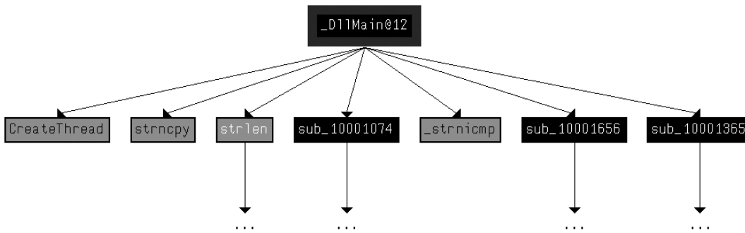
Figure 5-6L: Cross-reference graph for DllMain with a recursive depth of 1
